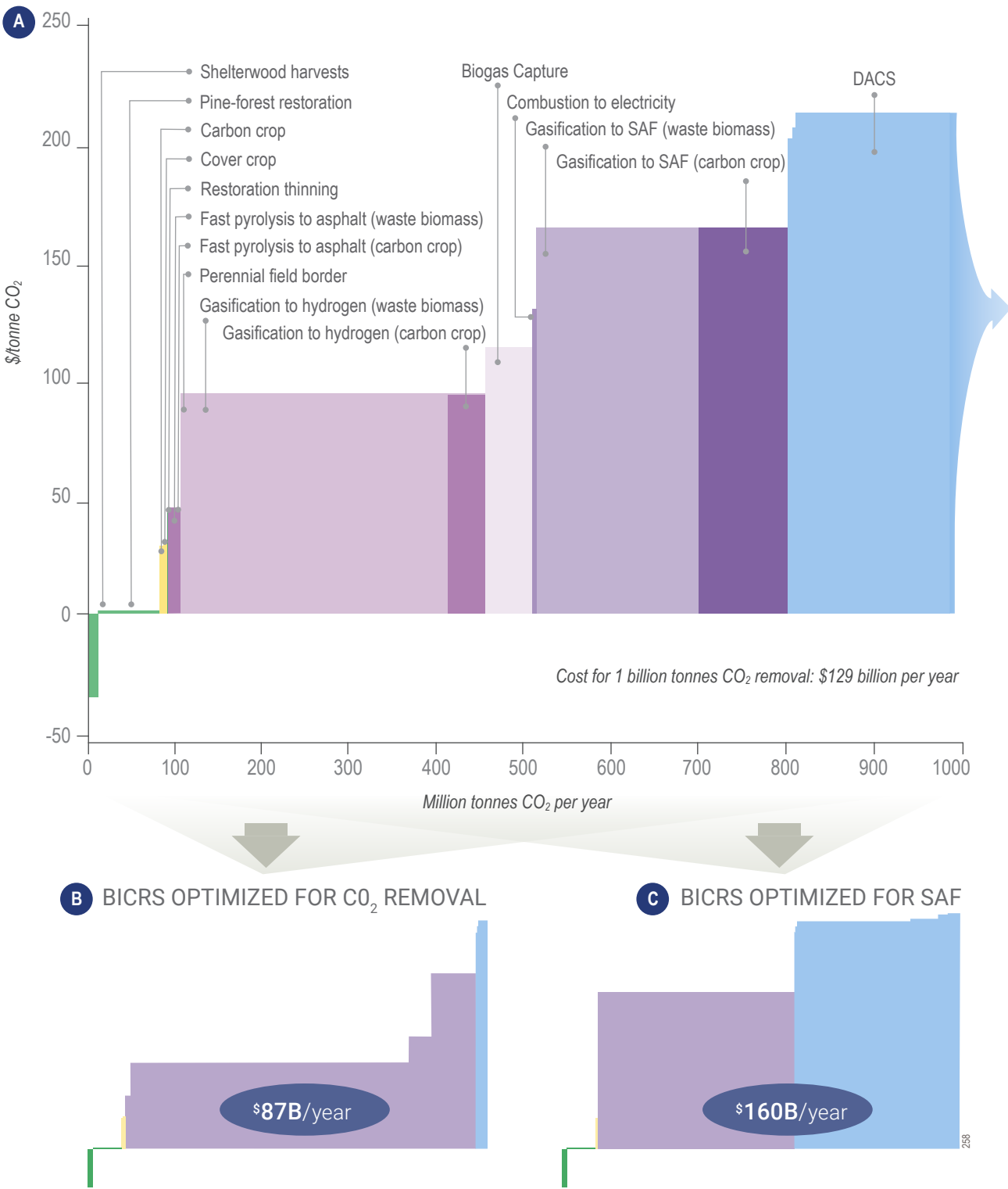
Figure ES-4. Representative 2050 supply curve for 1 billion tonnes of CO 2 removal per year in the United States, calculated from a high-resolution, county-level analysis. Amounts are ordered by estimated cost and constrained by resource availability, land use and energy supply. All costs include capital, operation, transportation, life-cycle costs and carbon impacts. Forest management potential (green) is calculated for only 3 regions of the US (northeast, western, southeast). For commodity-cropland soils (yellow), we focused on cover crops, perennial field borders, and perennial carbon crops. For BiCRS (purple), waste and crop biomass could be used for many national priorities—in (A), a subset of the biomass supply is allocated to sustainable aviation fuel (SAF) (17.5 billion gallons per year) and the remainder modeled to minimize carbon-removal cost; in (B) biomass use is optimized for CO 2 removal (with no SAF); in (C) we optimized for 28 billion gallons per year of SAF. The capacity for direct air capture with storage (DACs, blue) is larger than displayed; DACs technical potential is nearly 14 billion tonnes of CO 2 per year at less than $250/tonne. The integrated area of all bars gives the total cost for 1 billion tonnes of CO 2 removal per year.
