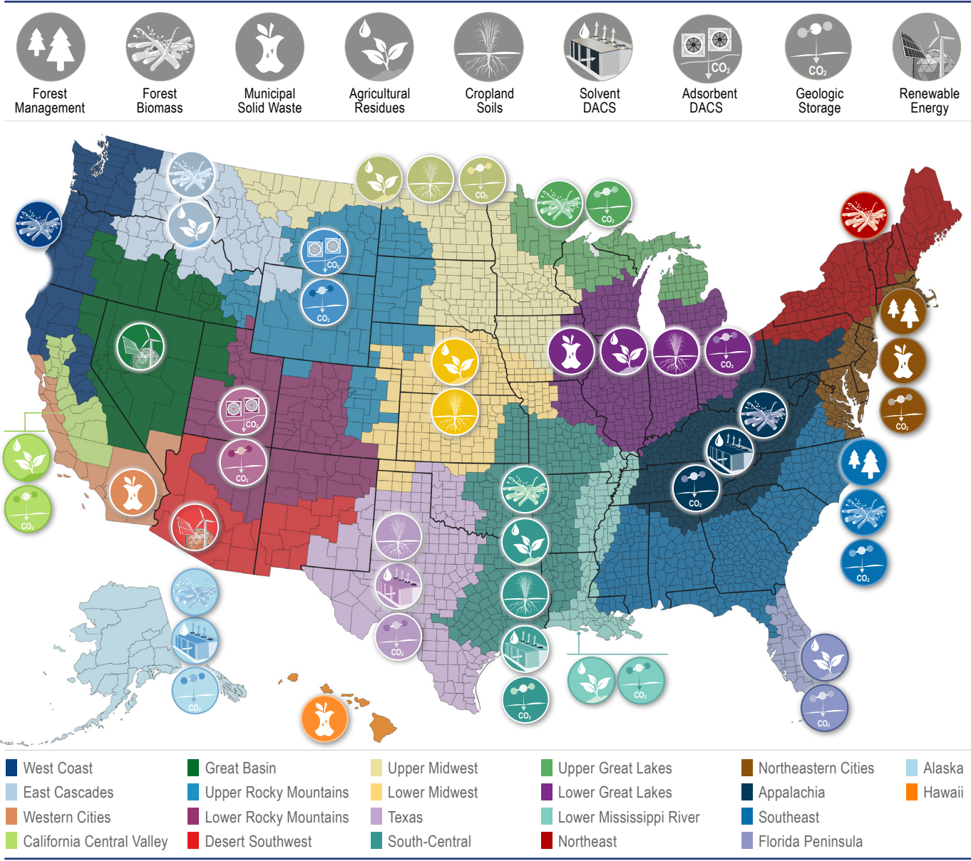
Figure ES-5. Regions map with county grouping defined by primary carbon-removal resources. The icons qualitatively highlight key regional resources that can contribute to CO 2 removal. We determined the regional groupings on a quantitative basis with qualitative boundary conditions. First, we assessed the primary above-ground carbon resources at a county level with a coarse boundary between forests, agriculture, urban, and other areas. Second, we evaluated geographic carbon-storage potential in forest biomass, cropland soils, and geologic reservoirs. Third, we analyzed cross-cutting factors, including watersheds, energy-generation capacity, and current and potential transportation resources. Fourth, we considered regional land ownership and environment and population health. Finally, we made judicious decisions about where to merge, divide, stretch, and contract each region based on the cohesive story that could be told, while incorporating boundary conditions (e.g. we required each region to be contiguous, including bodies of water).
